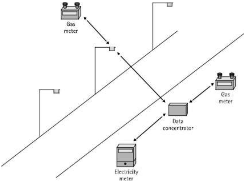
Fig. 5–1. A scenario using repeaters installed on streetlights
