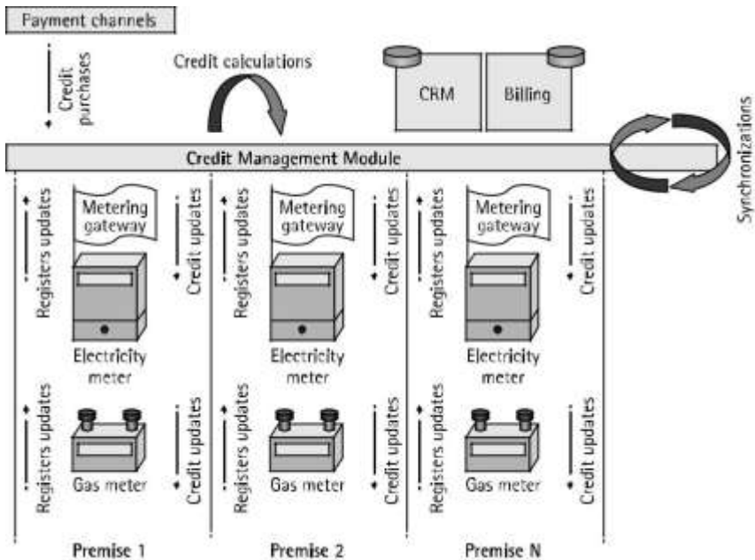
Fig. 2–3. Example of prepayment using centralized processing
