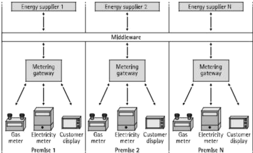
Fig. 2–28. In-home metering gateway separated from meters
