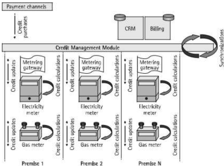
Fig. 2–4. A prepayment scenario using decentralized processing
