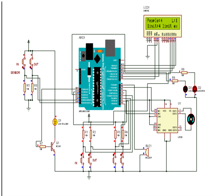
Fig. 11: Simulation Result Displaying the Maximum Number of Peoples in the Room
