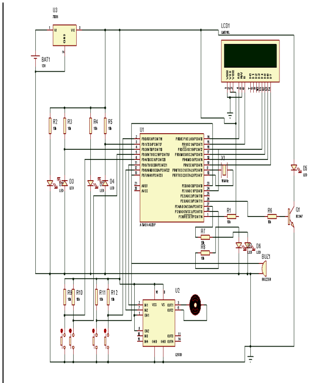
Fig. 3: Complete Circuit Diagram of the Visitors Counter with Gate Control and Automatic Room Light Controller (ON/OFF)
