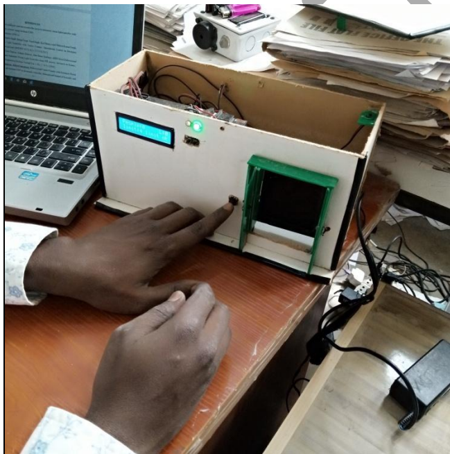
Fig. 8: Implemented Circuit Displaying the Process of Pressing the Entrance Door
