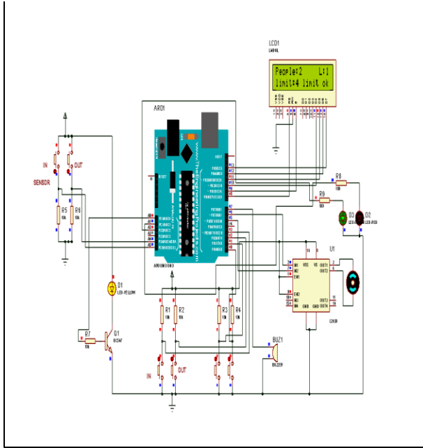
Fig. 9: Simulation Result Displaying Two Peoples are in the Room
