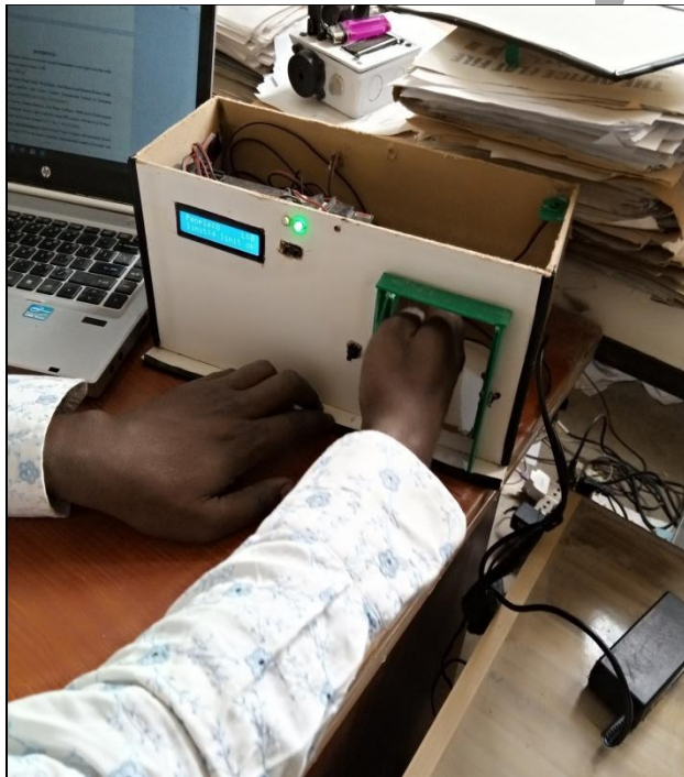
Fig. 10: Implemented Result on the Entrance Door
