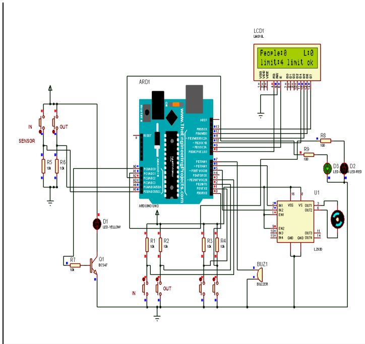
Fig. 7: Simulation Result Displaying Nobody is in the Room (people zero): Visitors Counter with Gate Control and Automatic Room Light Controller (ON/OFF)
